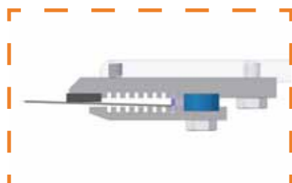
O5 LC-114-R creping blade holder, with ladder system
