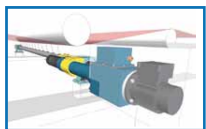
11 OSCILAN Oscillating shower, for wire and felt cleaning (15-30 bar)
