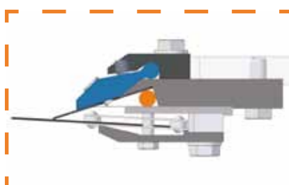
O1 Crepilan-C semi-flexible creping blade holder + Edge Fingers, with cartridge system (For Yankees with extreme crown)
