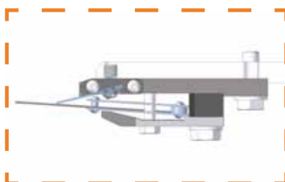
O4 LC-114-C creping blade holder, with cartridge system
