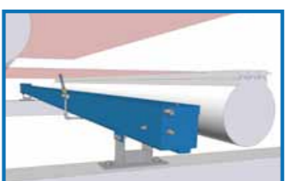
14 LANJET Shower, for wire and felt cleaning, with zone/spot cleaning system (15-30 bar)
