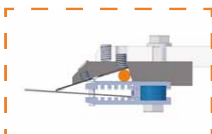
O3 Crepilan-R semi-flexible creping blade holder with ladder system
