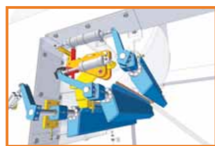
6 Creping Doctor with Automatic Alpha System
