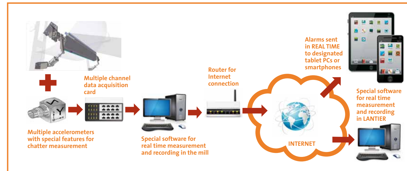
7 Anti-Chatter Creping Doctor Sensorized Diagnostic Platform for Creping
