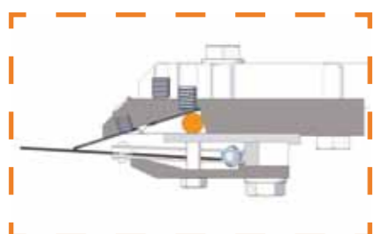
O2 Crepilan-C semi-flexible creping blade holder, with cartridge system
